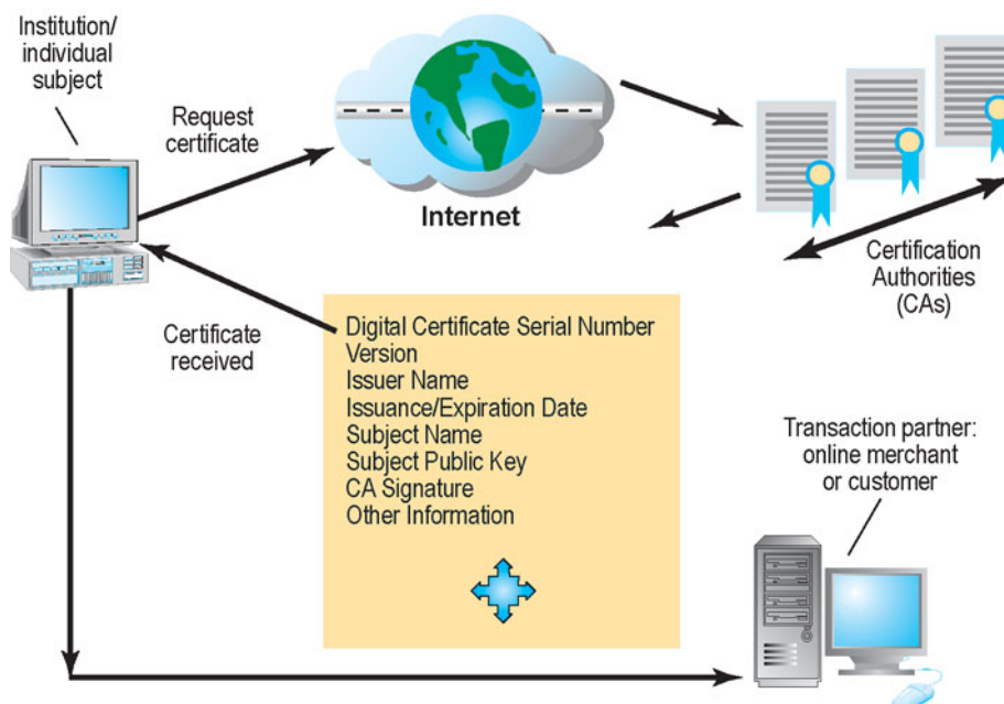
FIGURE 8.7 DIGITAL CERTIFICATES
